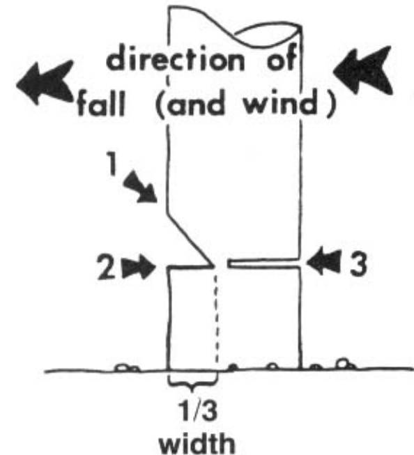
Chainsaw felling; note sequence of cuts.
